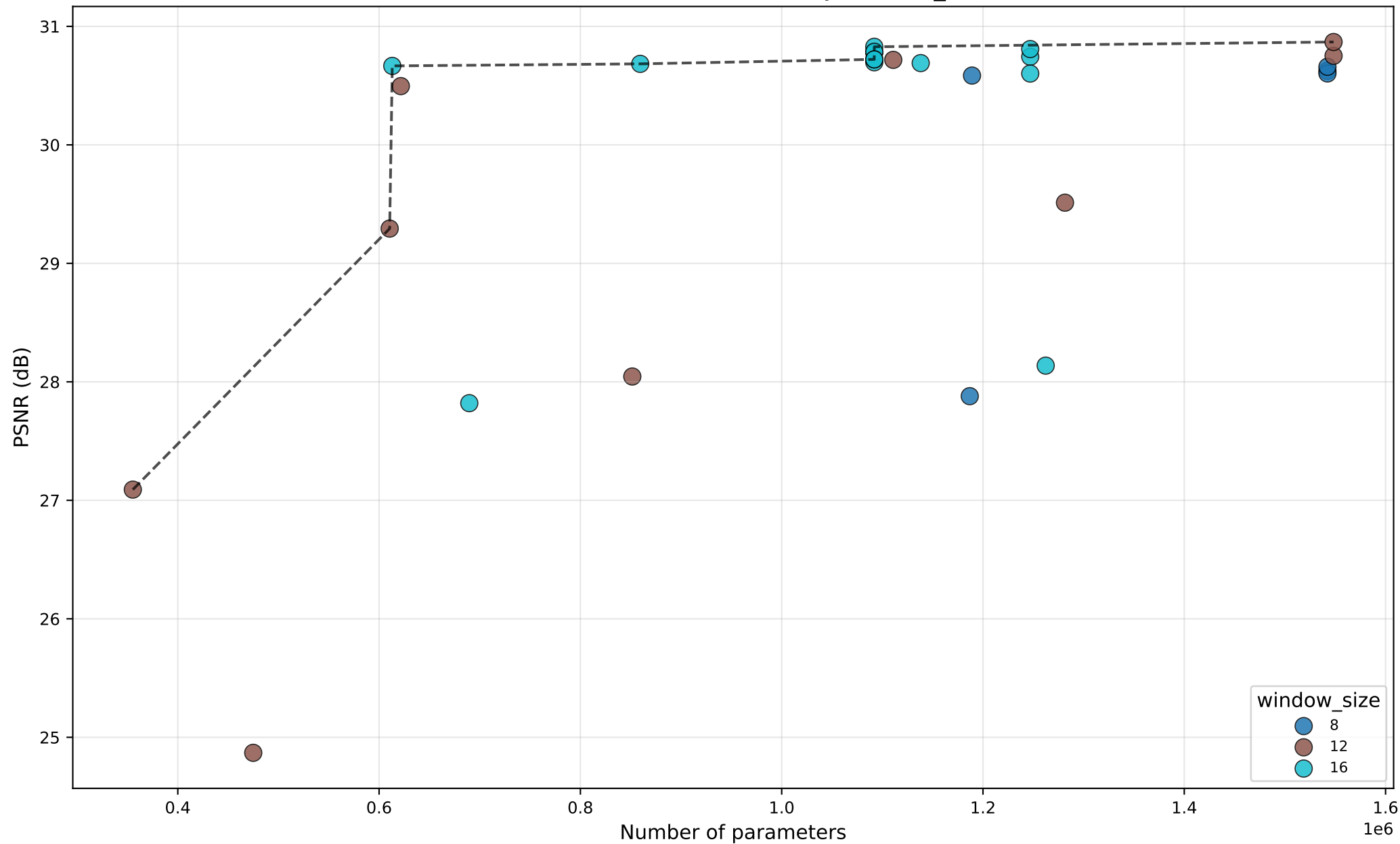
PSNR vs #Params — HAT — by window_size
